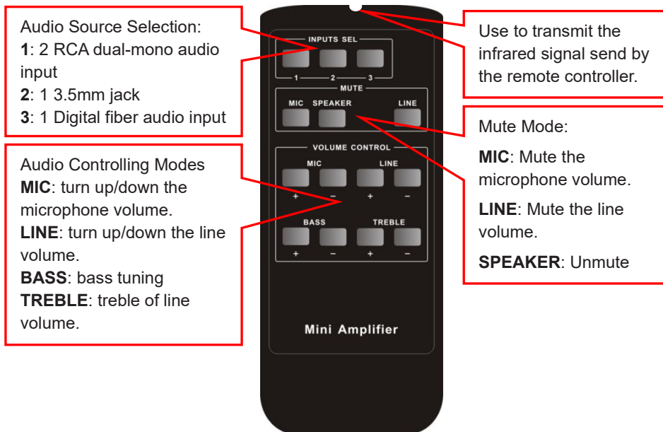
Figure 8 IR Remote
